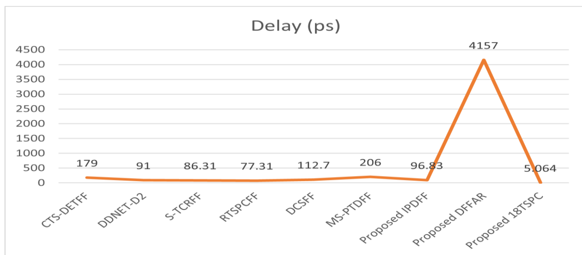
Fig.9: Comparison of Propagation Delay
