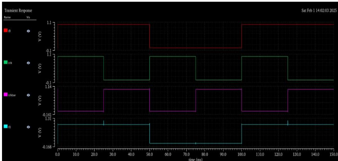
Fig 3: Input and Output Waveforms of PTIP-DETF
