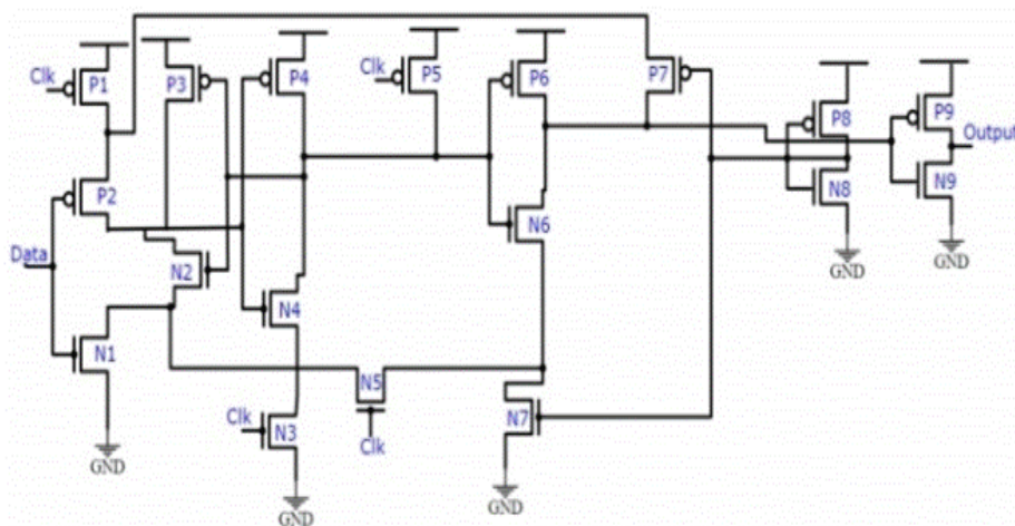
Fig. 6. Circuit of 18-TSPC D-FF
