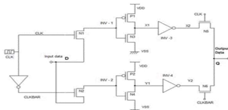
Fig. 1.Circuit of Proposed Pass Transistor Logic based ImplicitPulsed–Dual Edge Triggered Flipflop (IPDFF)
