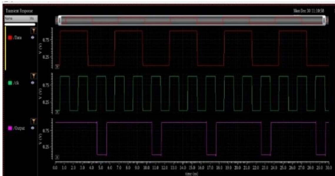
Fig. 8. Input and output waveforms of 18-TSPC D FF
