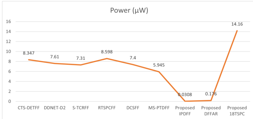
Fig.10: Comparison of Power Consumption
