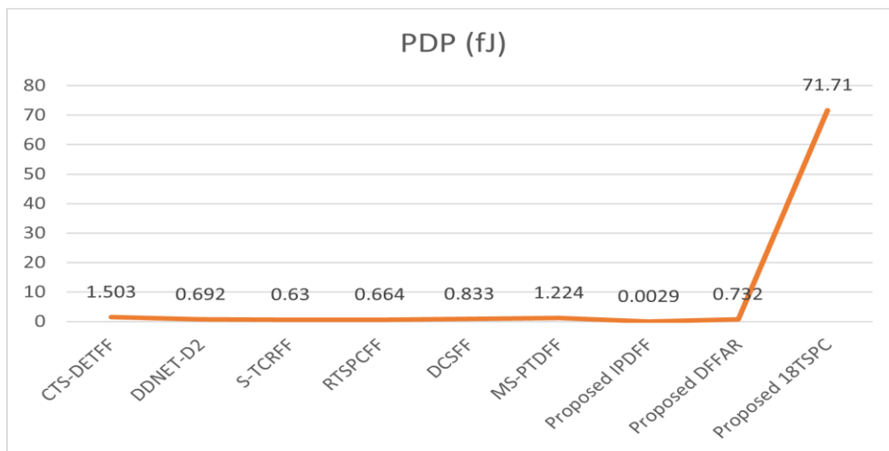
Fig.11: Comparison of energy (PDP)
