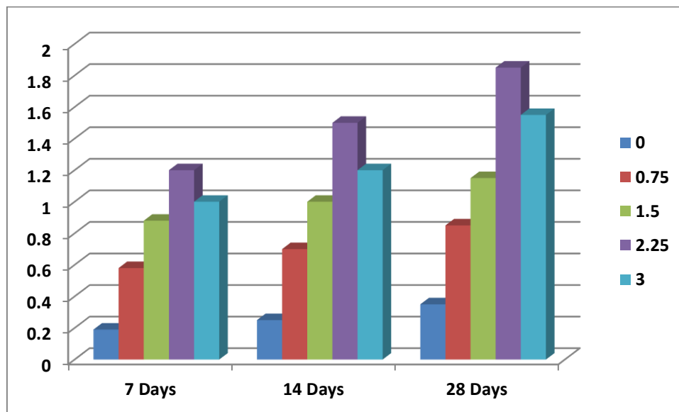
Figure 3: Effect of Coir Fibre on Flexural Strength (N/mm 2 )
