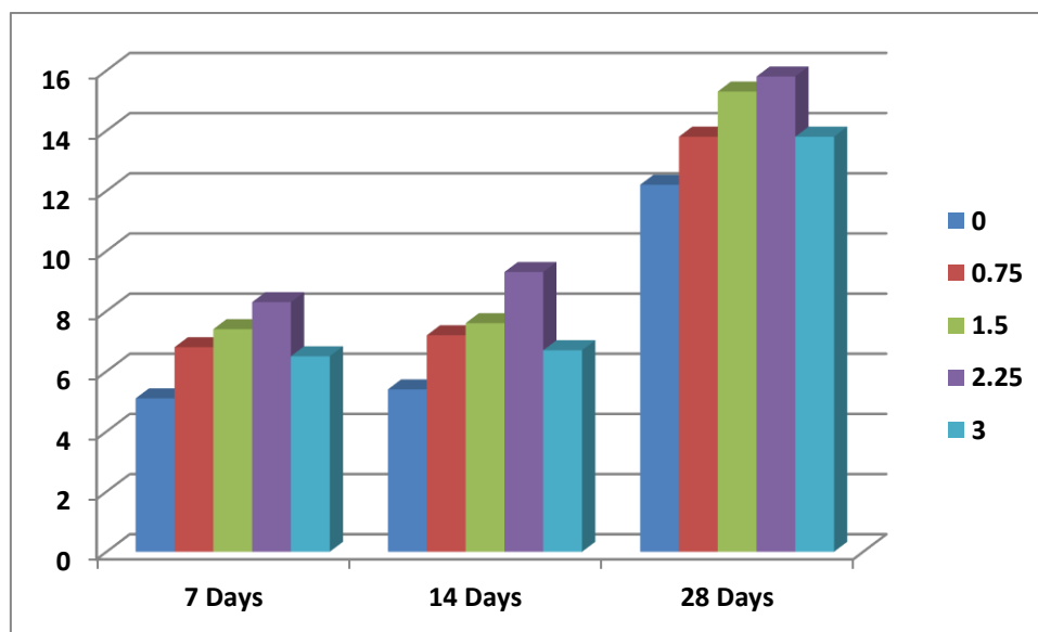
Figure 1: Coir Fibre Effect on Strength (N/mm 2 )
